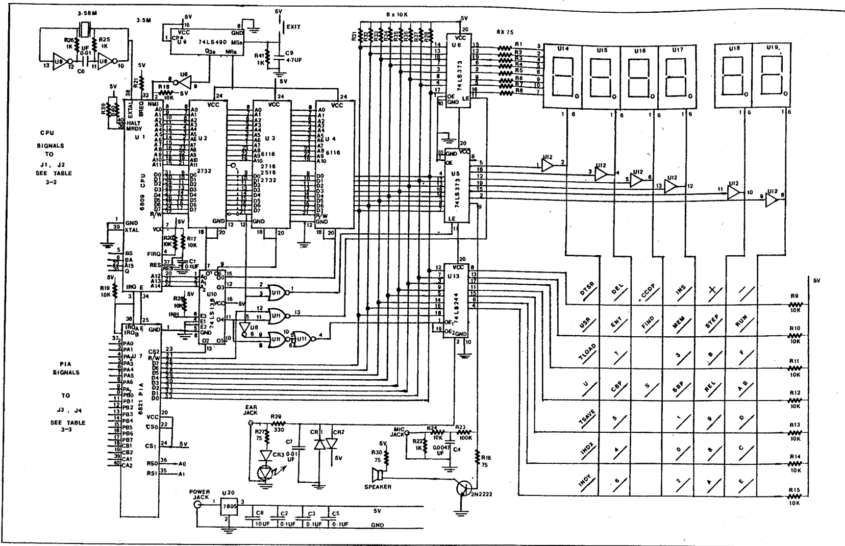
FIG 3-1 LS6809 CIRCUIT DIAGRAM
