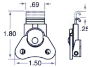
622-25 Basic catch
