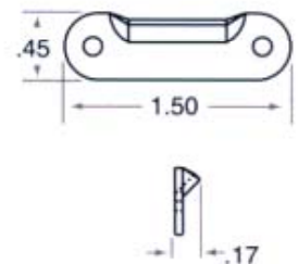
HS622-03 Concealed Strike
