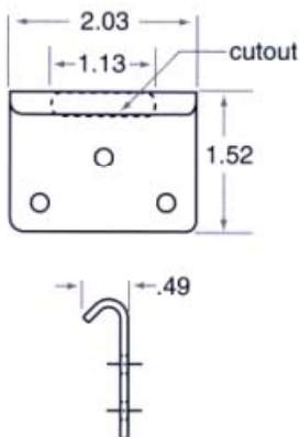
HS603-11 Large Strike
