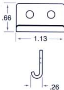
HS624-01 Medium Strike
