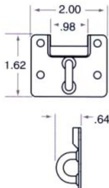
HS603-12 Used with 623-81
