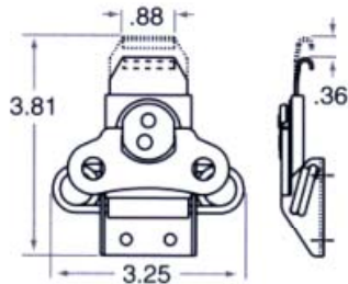
623-32 Base spring allows for misalignment between catch and strike
