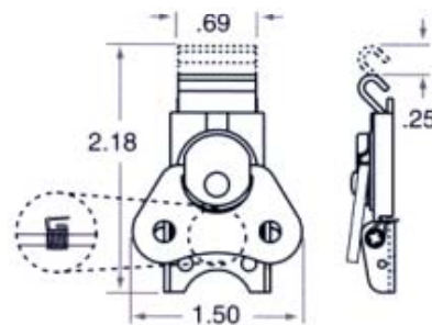
622-71 Kick-out spring (catch stays out of the way when unlatched)
