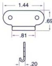
HS622-01 Small Strike
