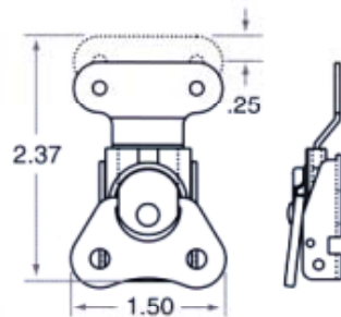
622-47 Hinged turn (integrated strike)
