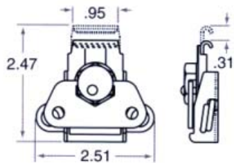
624-42 Base spring allows for misalignment between catch and strike, hexagonal cap
