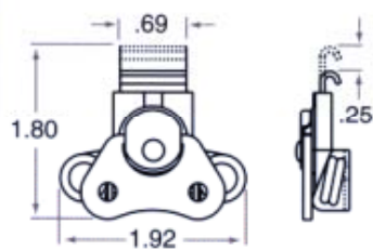
622-22 Base spring allows for misalignment between catch and strike
