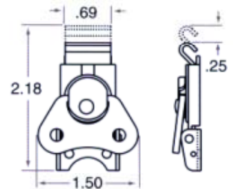
622-70 Upturned hook (low profile)
