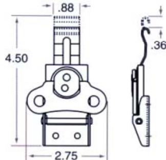
623-81 Can be used with a padlock
