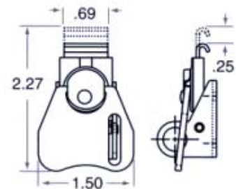
622-80 Can be used with a padlock
