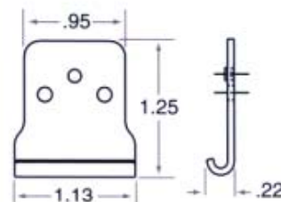
HS622-02 Small Strike
