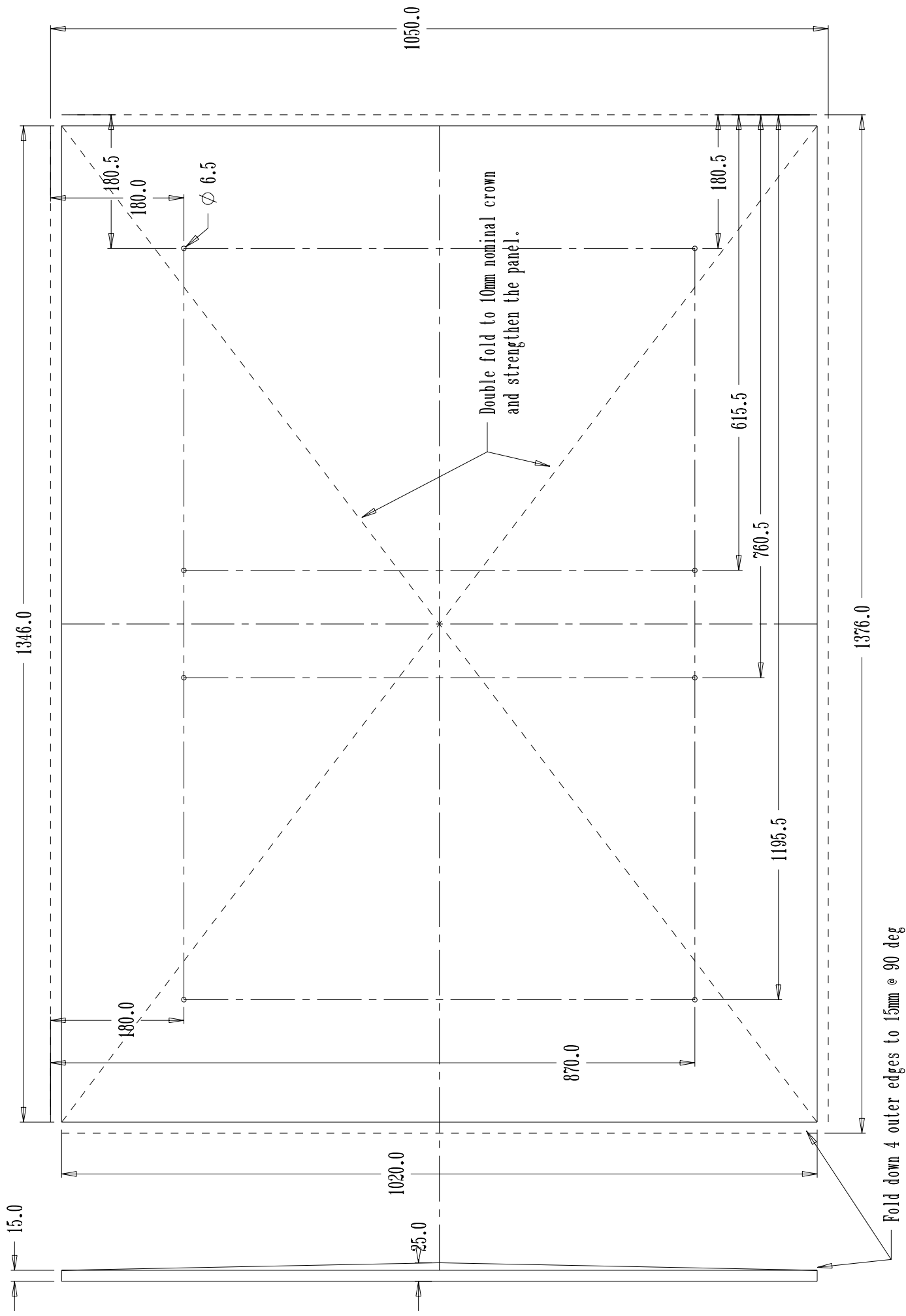
Top Cover for Double Rack - 1mm Steel (Zinc/Ally coat)
