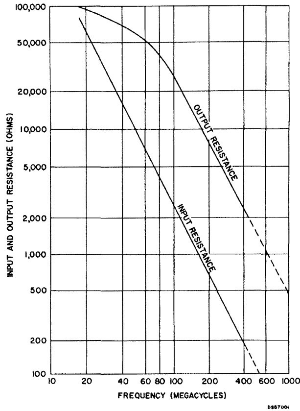
Figure 1—Input and output resistance vs frequency
